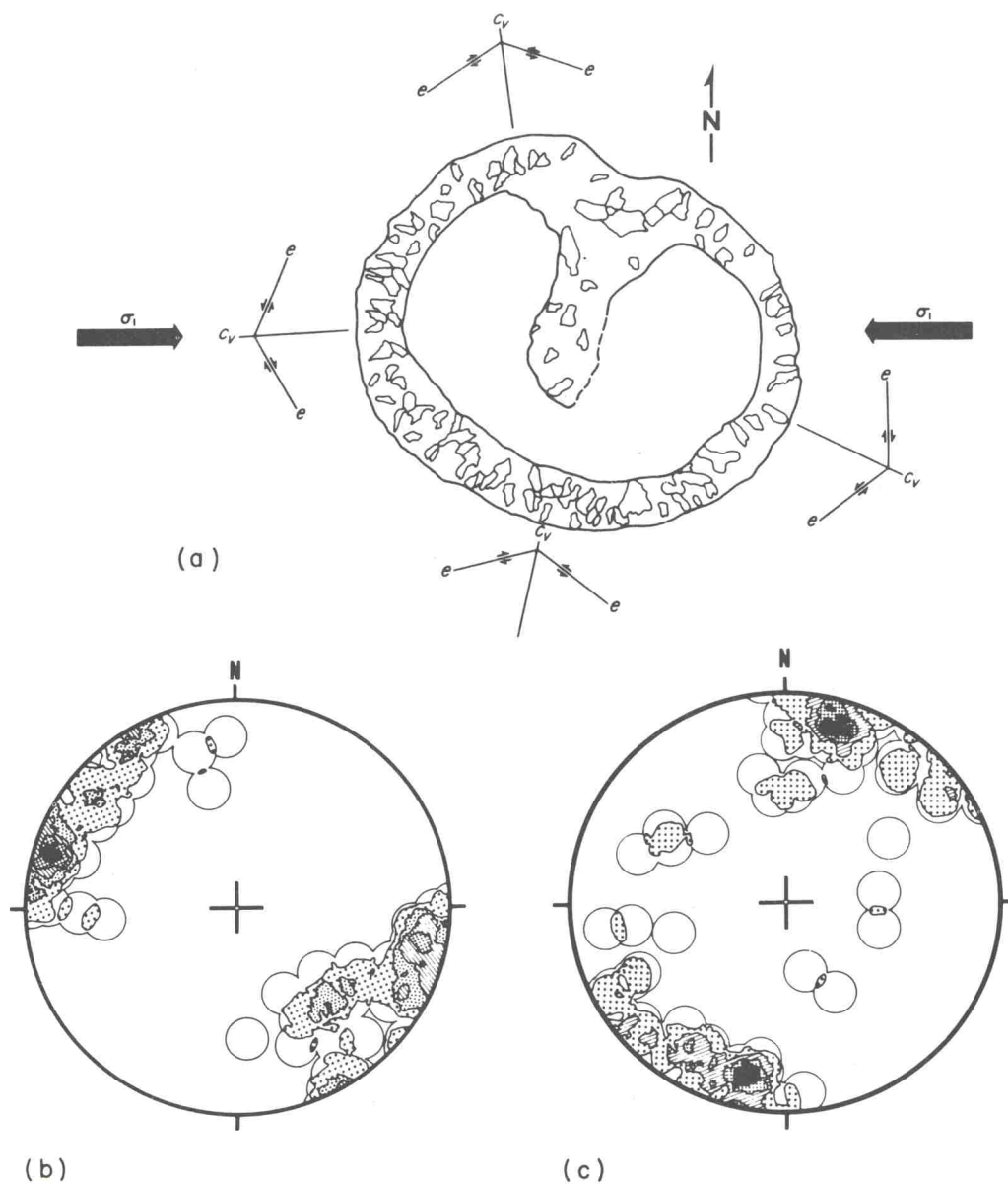
Fig. 29—Petrofabric analysis of calcite twin lamellae in the gastropod shell. (a) Approximate orientations of two e twin planes and the c_v in calcite crystals at four points within the gastropod shell. With respect to an assumed east-west greatest principal compression, the grains along the north and south sides of the shell are favorably oriented for twinning because of the sense of shear on the twin planes, whereas those on the east and west sides are unfavorably oriented (from Friedman and Conger, Ref. 112, Fig. 4). (b) Diagram illustrating the orientation of 70 compression axes derived from grains with high e_1 lamellae spacing index. Plane of the diagram is parallel to bedding with north as indicated for bedding unfolded. Contours are at 1.4, 2.9, 5.7, 8.6, 11.4, and 14.3 per cent per 1 per cent area, 15.7 per cent maximum (from Friedman and Conger, Ref. 112, Fig. 8b). (c) Diagram illustrating the orientations of 70 extension axes derived from same grains as in (b). Diagram oriented same as in (b). Contours are at 1.4, 2.9, 5.7, 8.6, and 11.4 per cent per 1 per cent area, 14.3 per cent maximum (from Friedman and Conger, Ref. 112, Fig. 9b).
